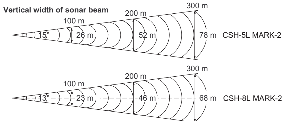
Depth, detection range and tilt angle
