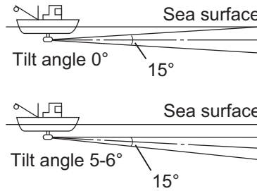
Tilt angle and surface fish (example: CSH-5L MARK-2)
